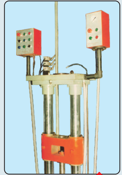
Vertical Pull Type Broaching Machine
